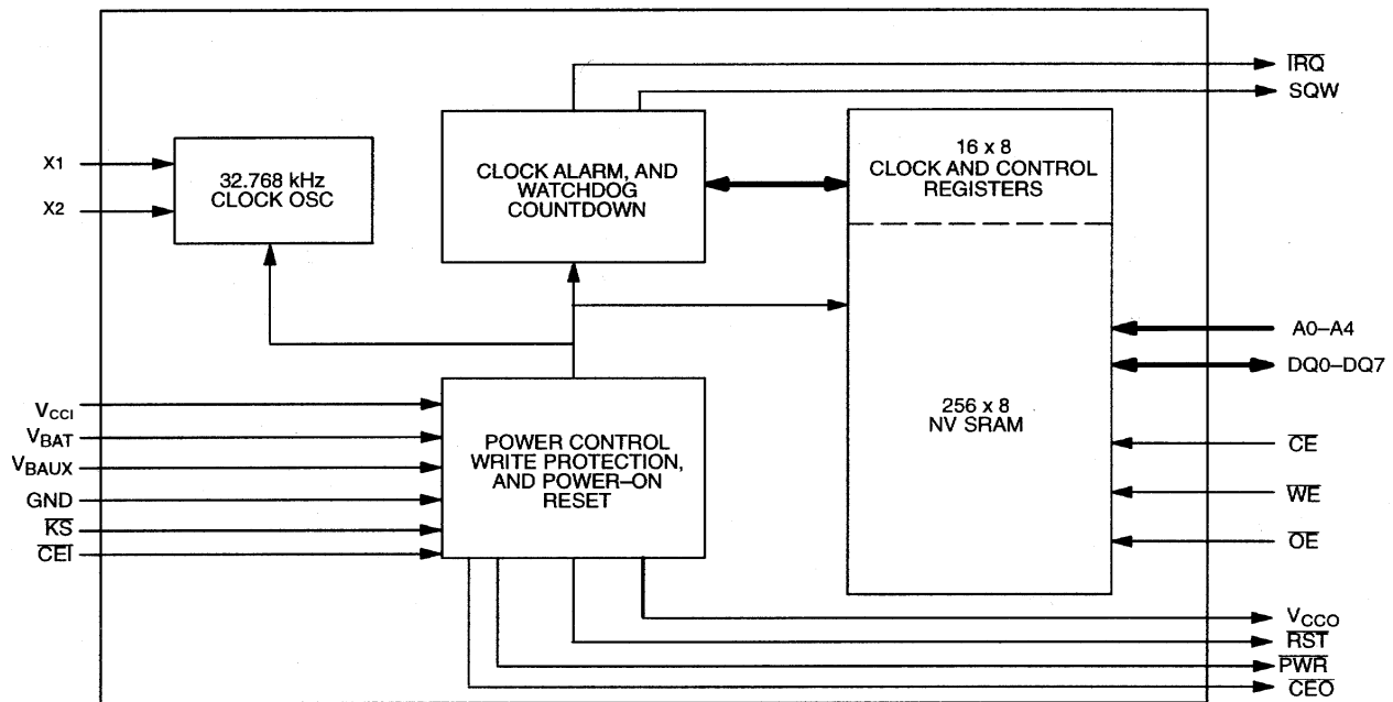
DS1500/DS1510 BLOCK DIAGRAM Figure 1
